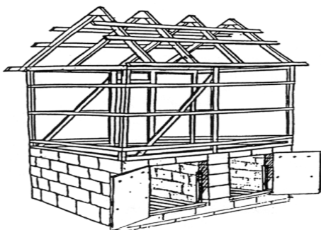
Fixed chamber batch used in Tonga, Kiribati and Australia
