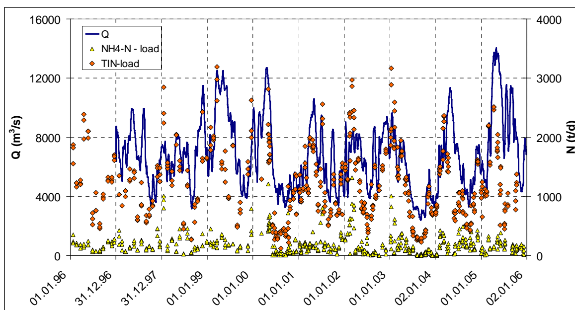
Figure 2: TIN and \text{NH}_4\text{-N} -loads and Danube discharges at Reni from 1996-2005
