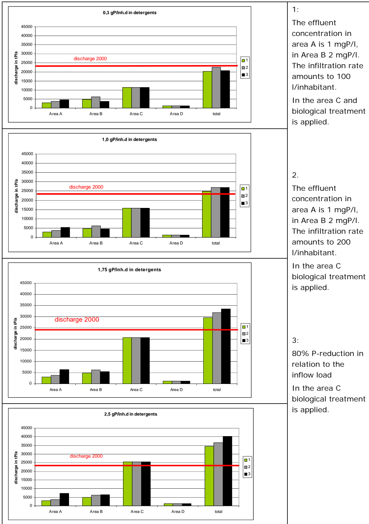
Figure 25: P-emissions in different settlement categories and different variants
