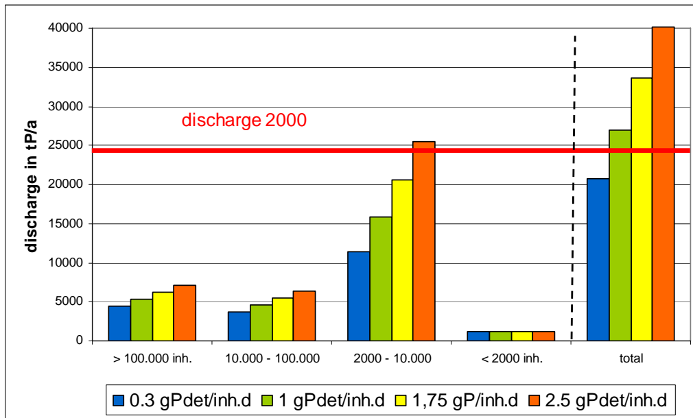
Figure 28: P-discharge of Variant 3: 80% P-reduction in relation to the inflow load. In the area C biological treatment is applied.
