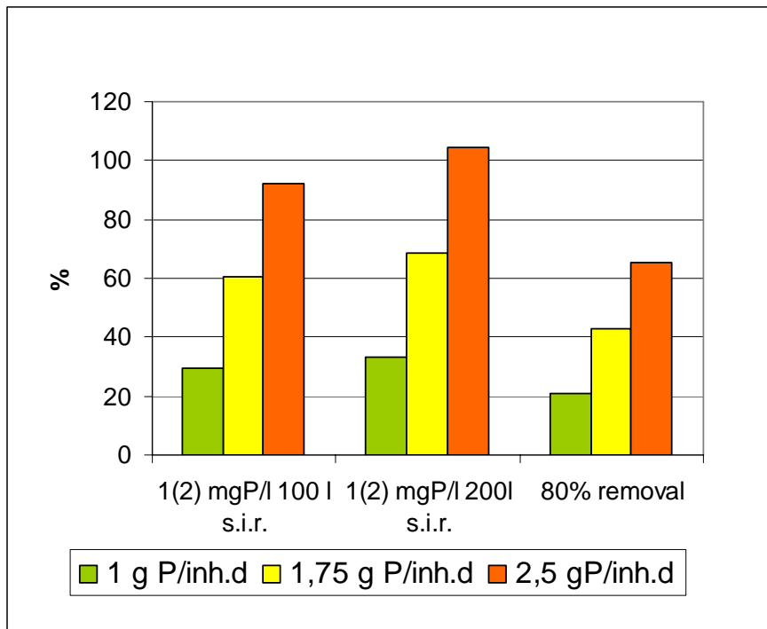
Figure 22: Additional need for precipitants of 3 variants in % of the “Zero laundry detergent Scenario” (0.3 g P/inh.d from detergents)
