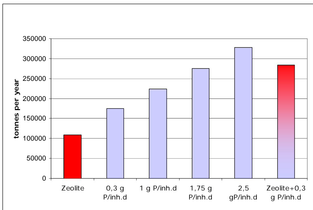
Figure 21: Increase of sludge dry matter due to P-precipitation in treatment plants above 10.000 pe or due to the replacement of P-containing laundry detergents by Zeolite in t/a (mean of the variants are used)
