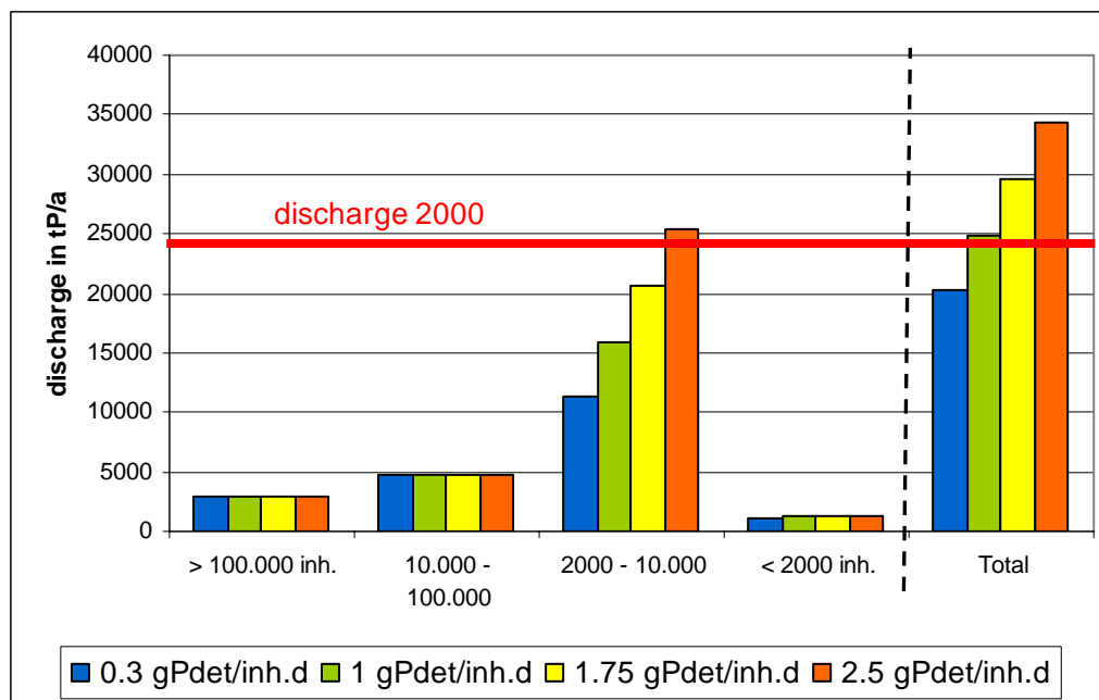
Figure 26: P-discharge of Variant 1: The effluent concentration in area A is 1 mgP/l, in Area B 2 mgP/l. The infiltration rate amounts to 100 l/inhabitant. In the area C biological treatment is applied.
