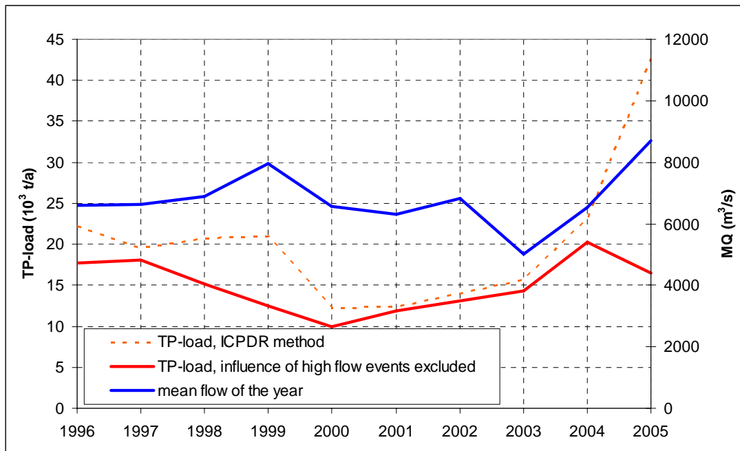
Figure 10: Yearly TP-loads and Danube discharges at Reni from 1996-2005
