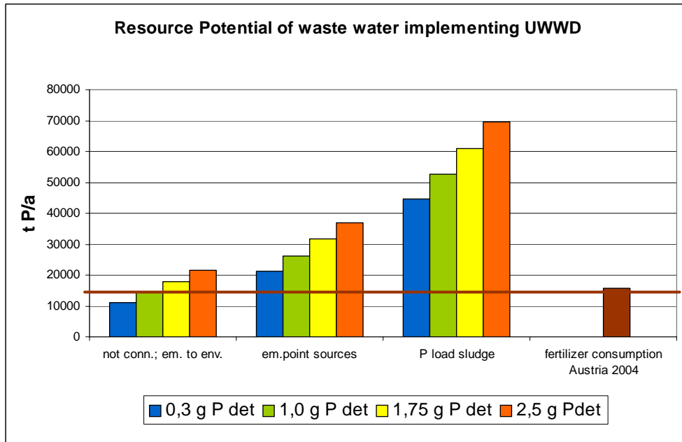
Figure 20: Amount of P in various P-flows in comparison with the P-fertilizer consumption in Austria 2004
