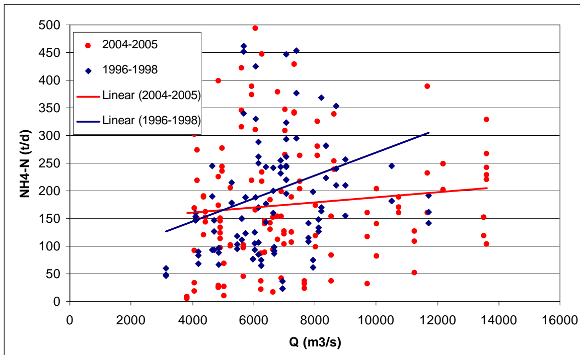
Figure 6: NH 4 -N-loads and river discharges of the Danube River at Reni
