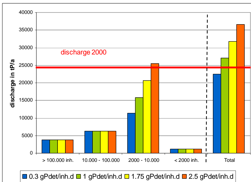
Figure 27: P-discharge of Variant 2: The effluent concentration in area A is 1 mgP/l, in Area B 2 mgP/l. The infiltration rate amounts to 200 l/inhabitant. In the area C biological treatment is applied.
