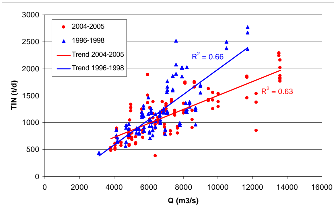
Figure 4: TIN-loads and river discharges of the Danube River at Reni
