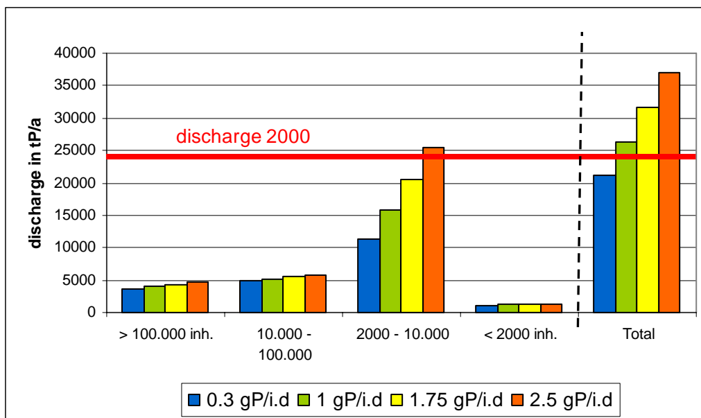
Figure 18: Mean P-discharge in different scenarios in tP/a.
