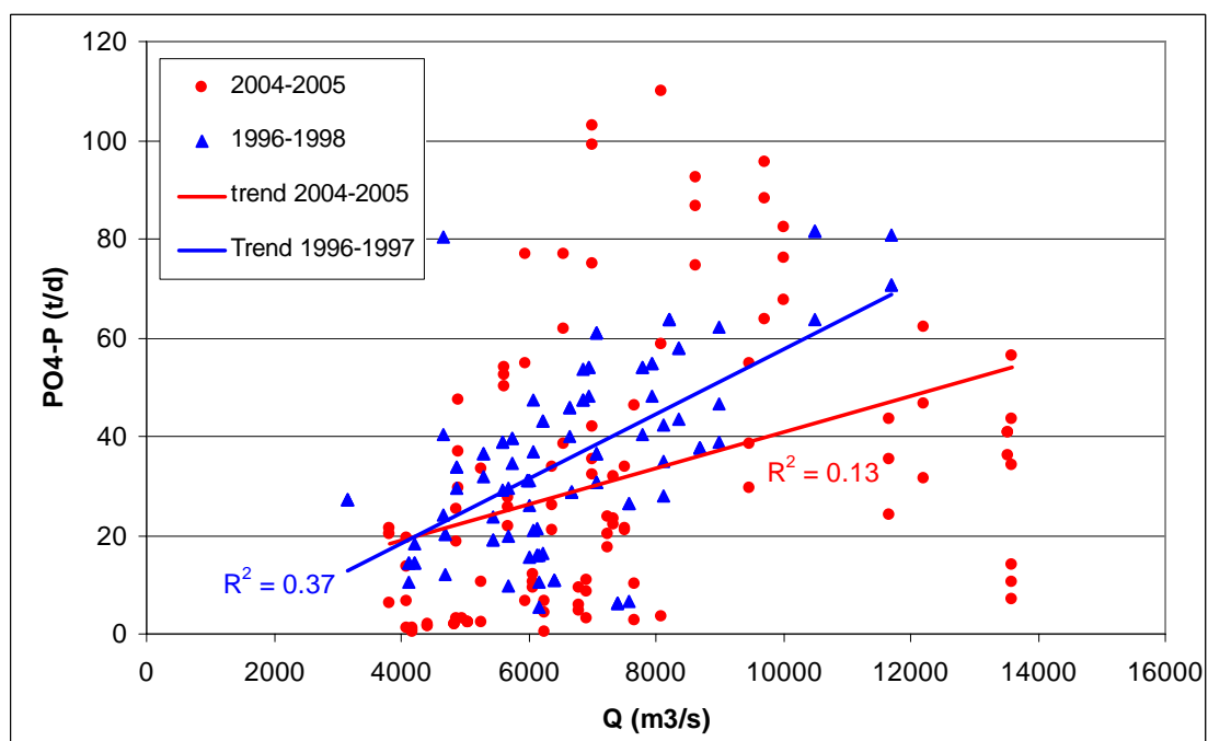
Figure 11: \text{PO}_4\text{-P} -loads and river discharges of the Danube River at Reni
