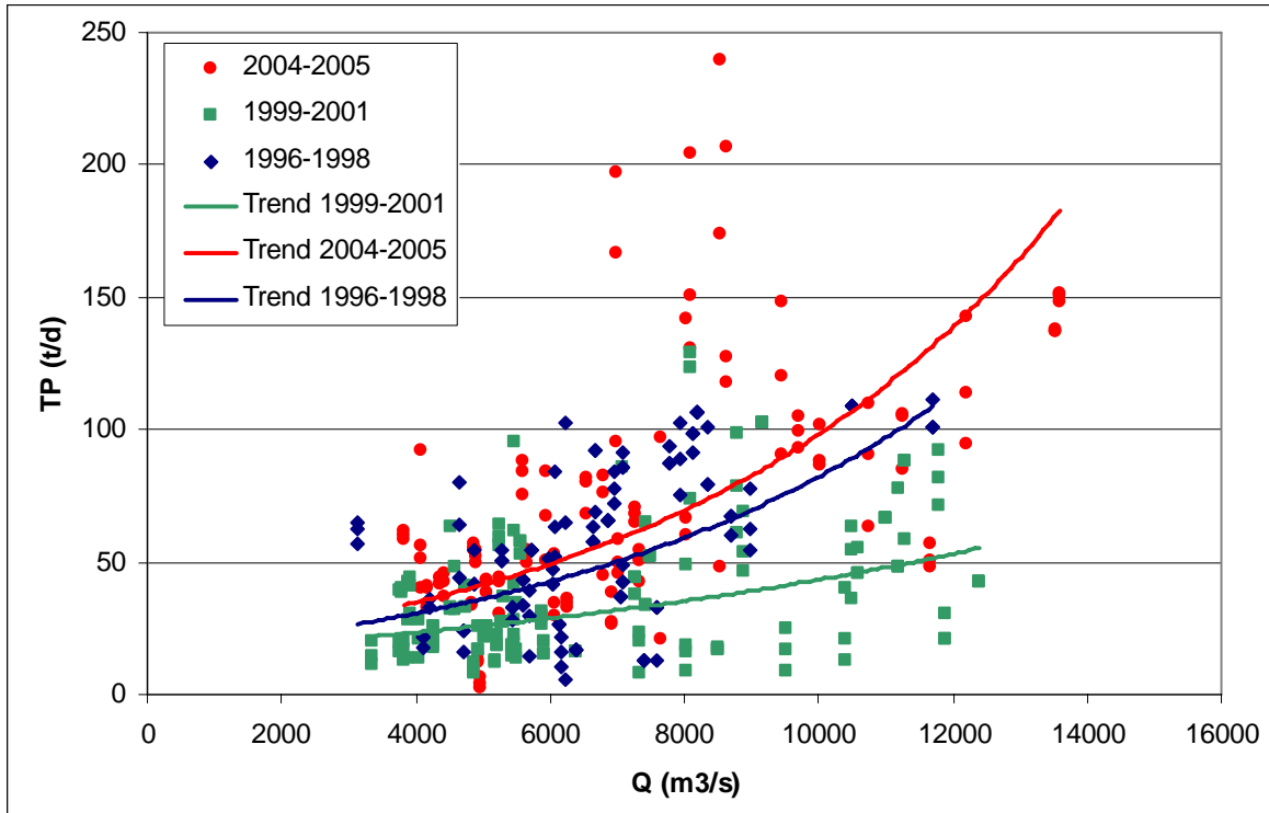
Figure 9: TP-loads and river discharges of the Danube River at Reni
