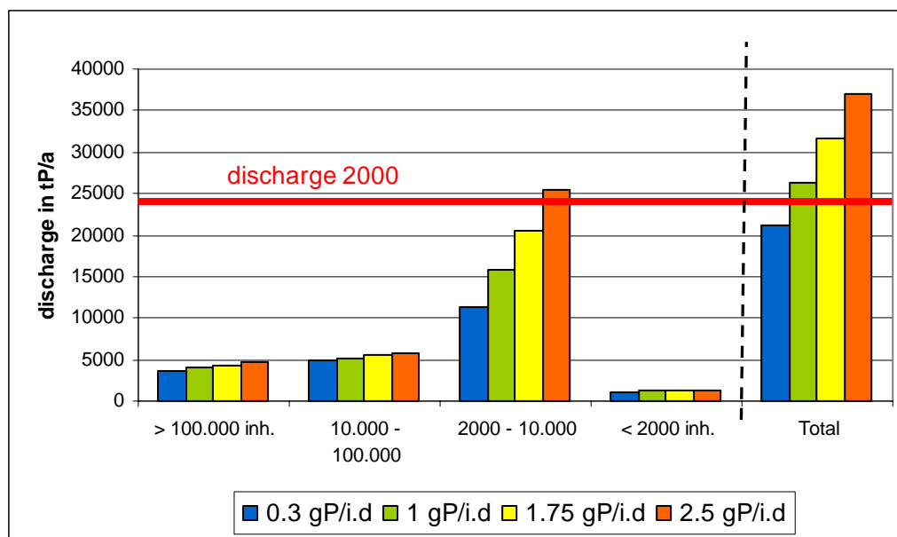
Figure 1: Mean P-discharge in different scenarios in tP/a.
