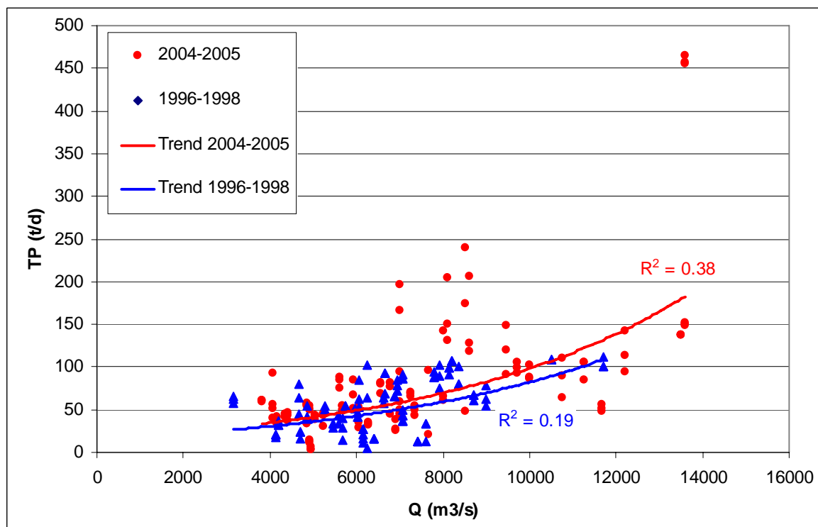
Figure 8: TP-loads and river discharges of the Danube River at Reni
