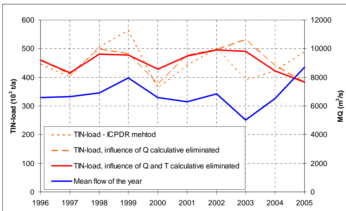
Figure 5: Yearly TIN loads and Danube discharges at Reni from 1996-2005
