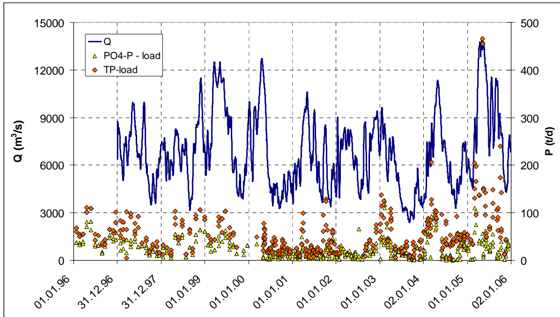
Figure 7: TP and PO 4 -P-loads and Danube discharges at Reni form 1996-2005
