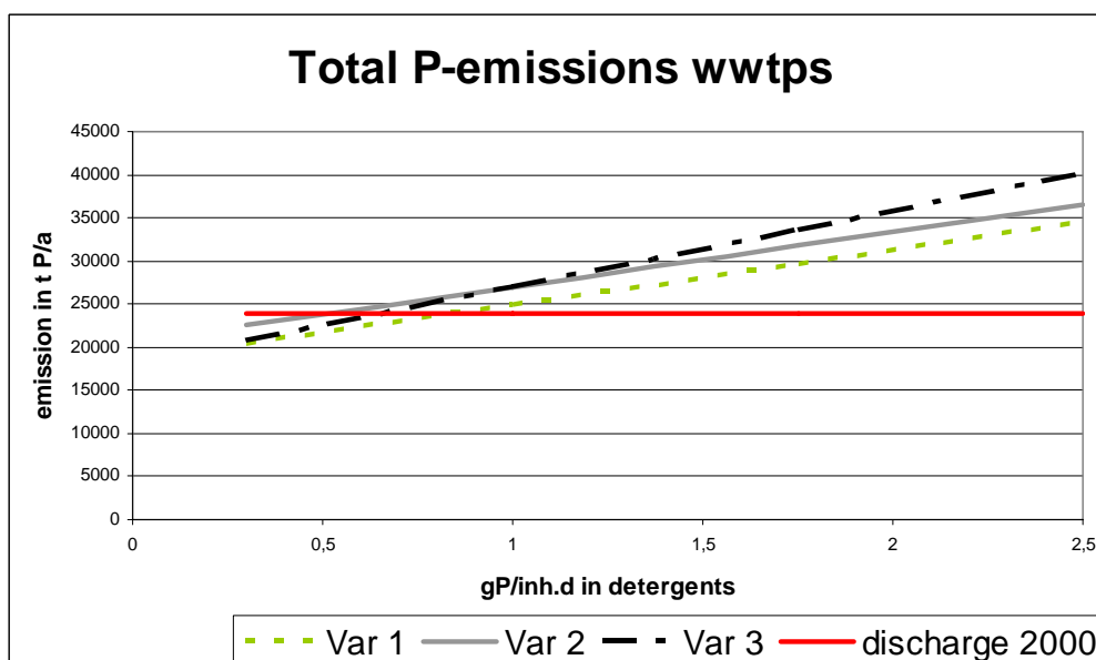
Figure 19: P-emissions from WWTPs of the 3 variants considered
