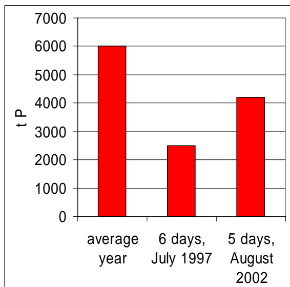
Figure 24: P-flow at high flow: Danube at Vienna
