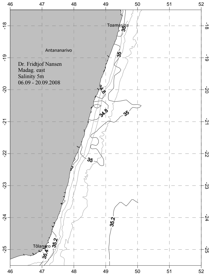
Figure 3.21 Horizontal distribution of salinity at 5 m on the south-eastern shelf of Madagascar based on data recorded underway.
