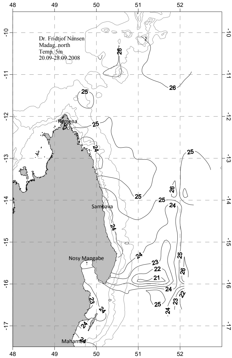
Figure 3.19 Horizontal distribution of sea temperature at 5 m on the north-eastern shelf of Madagascar based on data recorded underway
