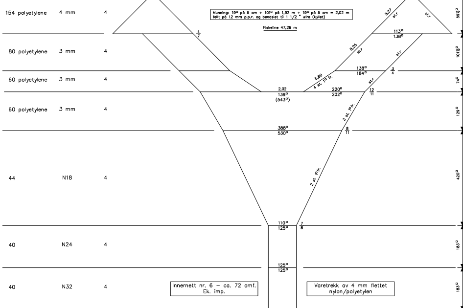
Design of the trawl used.
