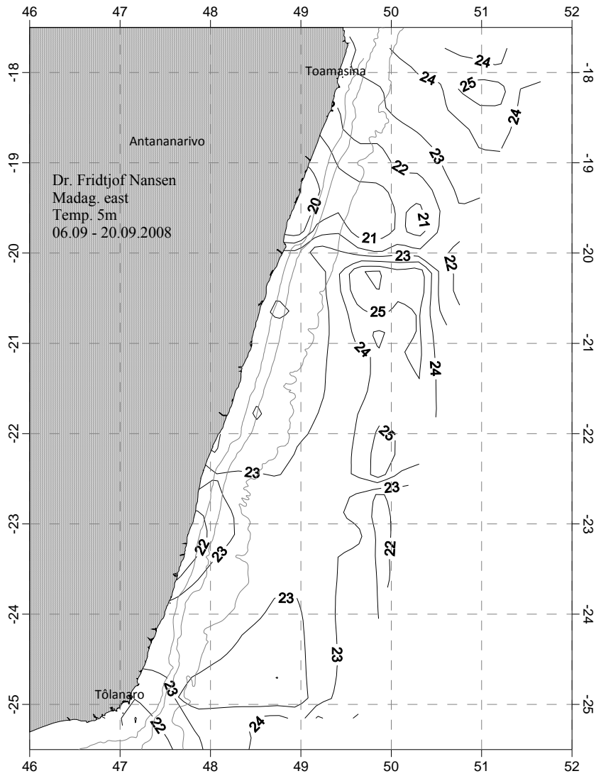
Figure 3.18 Horizontal distribution of sea temperature at 5 m on the south-eastern shelf of Madagascar based on data recorded underway.
