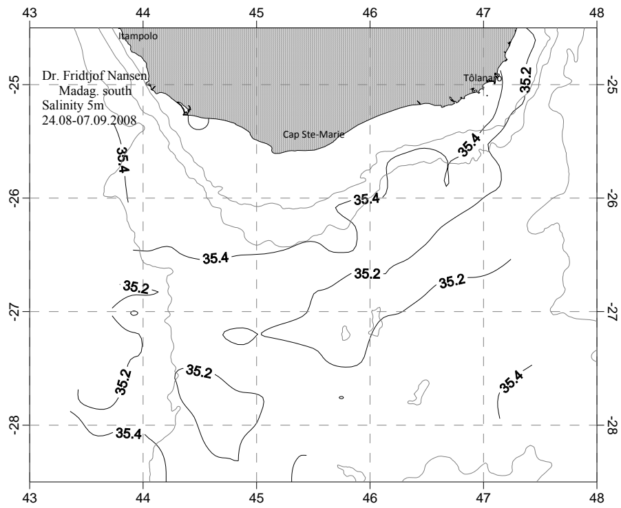
Figure 3.20 Horizontal distribution of salinity at 5 m on the Southern shelf of Madagascar based on data recorded underway.
