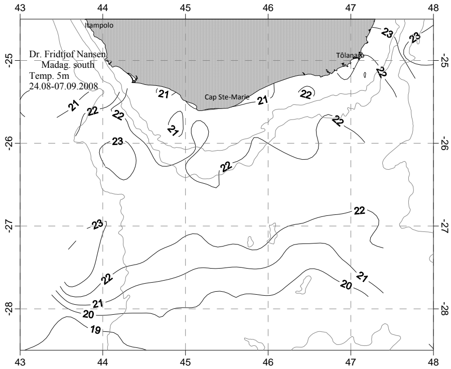
Figure 3.17 Horizontal distribution of sea temperature at 5 m on the Southern shelf of Madagascar based on data recorded underway.
