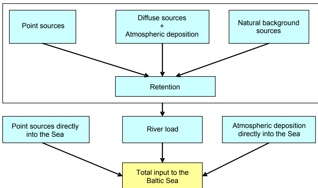
Figure 2-3. Sources of nutrients within the Baltic Sea catchment area (HELCOM, 2005).
