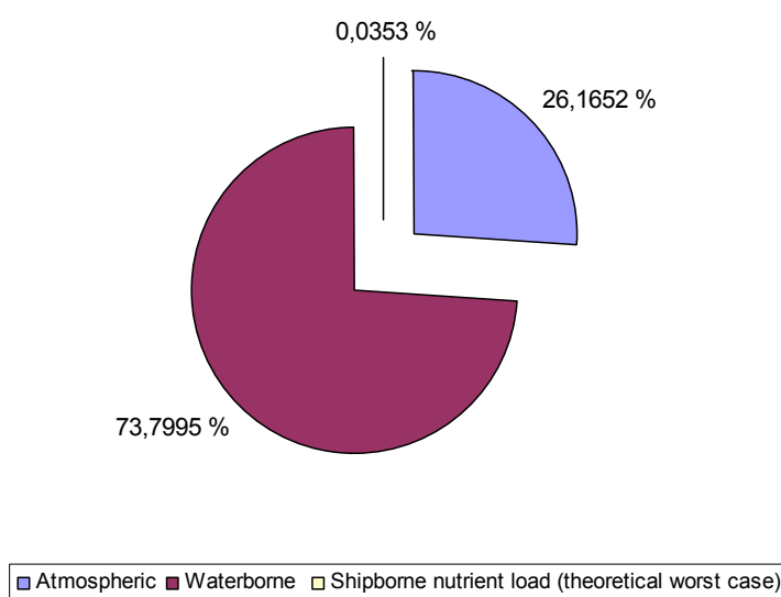
Figure 7-1. Total nitrogen input into the Baltic Sea
