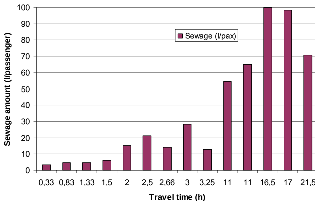
Figure 3-2. Waste water production vs. travel time.
