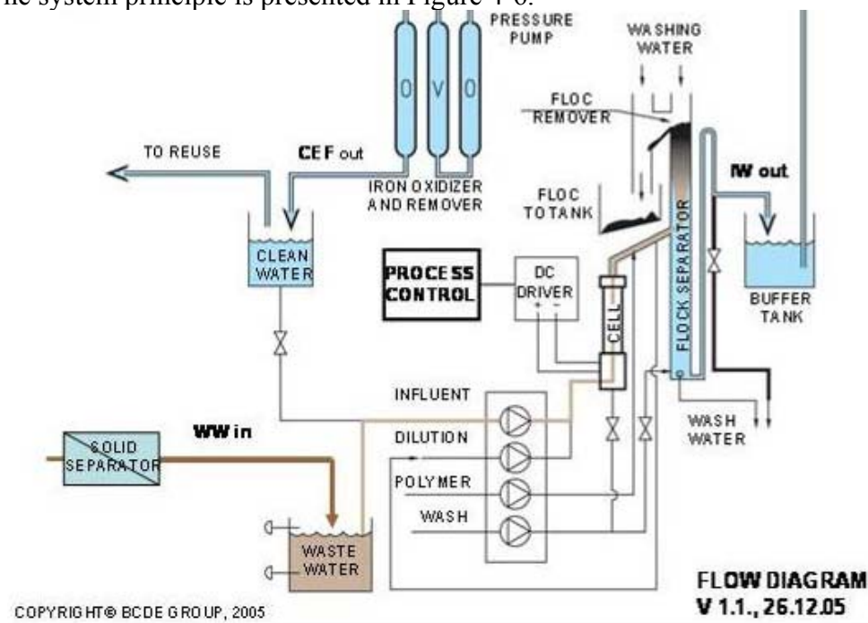
Figure 4-6. The principle of ECO-H2O™ water purifier (Dynamic Design, 2006).
