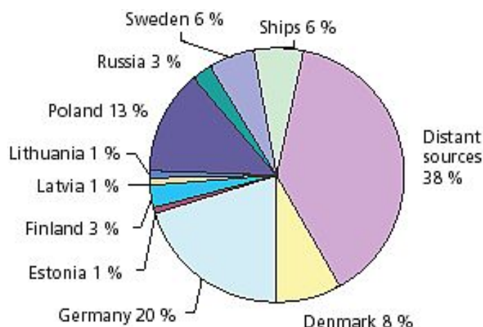
Figure 7-5. Proportion of atmospheric deposition of nitrogen in the Baltic Sea by HELCOM contributions in 2000. Note that the data ships' emissions only exist for the year 1990 and the same values have been used for all subsequent years (HELCOM, 2005).
