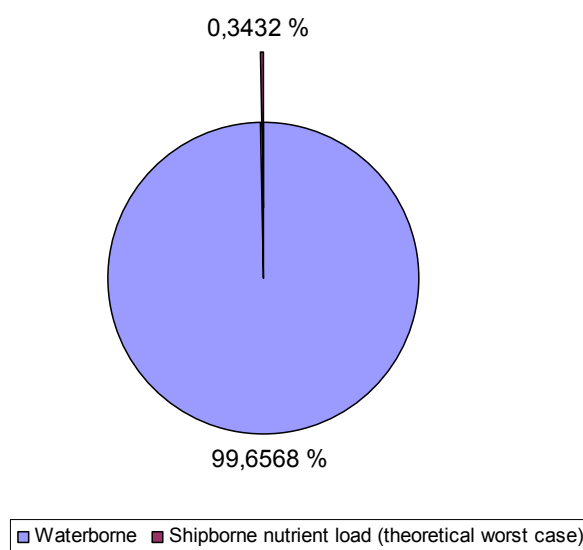
Figure 7-1. Total nitrogen input into the Baltic Sea
