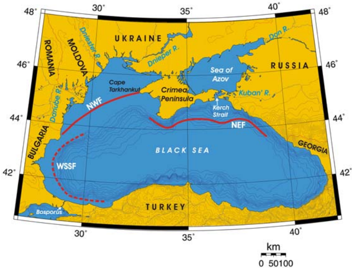
Figure V-8.1. Fronts of the Black Sea LME. NEF, Northeast Front; NWF, Northwest Front; WSSF, West Shelf-Slope Front (after Belkin 2009).
