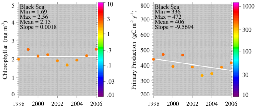
Figure V-8.3 Black Sea LME trends in chlorophyll a (left) and primary productivity (right), 1998-2006. Values are colour coded to the right hand ordinate. Figure courtesy of J. O'Reilly and K. Hyde. Sources discussed p. 15 this volume.
