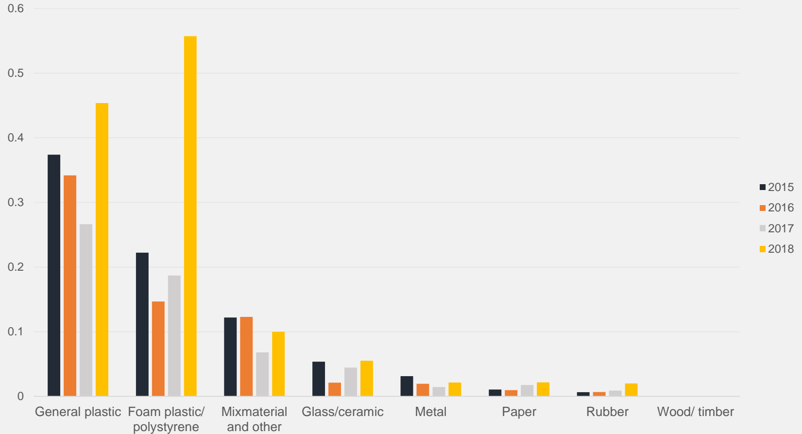
2015 - 2018 annual count accumulation rate of beach litter materials in Chinese coastline
