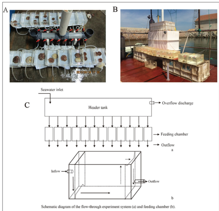
FIG. 1-4 The photo (A, B) and schematic diagram (C) of the filtration rate measurement device in situ for bivalves.
